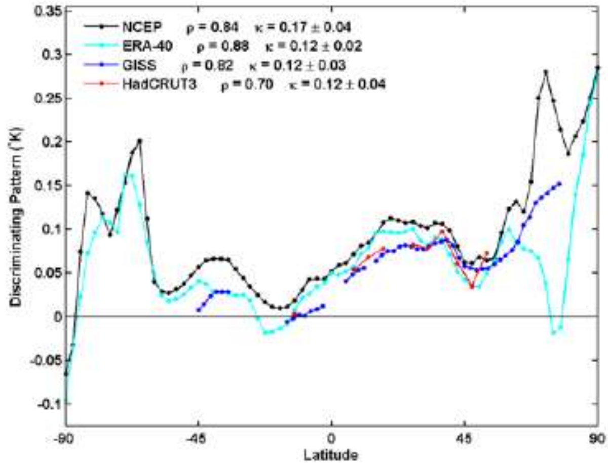
Zonal mean spatial pattern that best distinguishes solar max years from the solar min years
