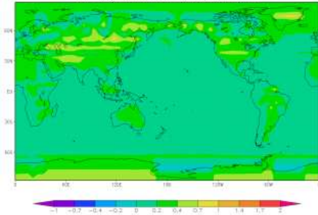
IAP RAS CM, annual (max)-(min), K
