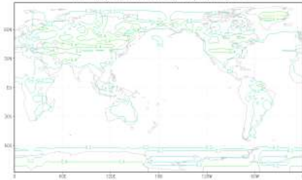
IAP RAS CM, annual (max)-(min), K
